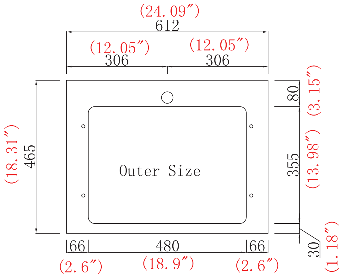
Top View
